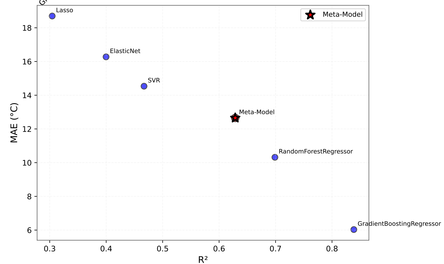
D: Performance Summary (Lower MAE, Higher R 2 is Better)
