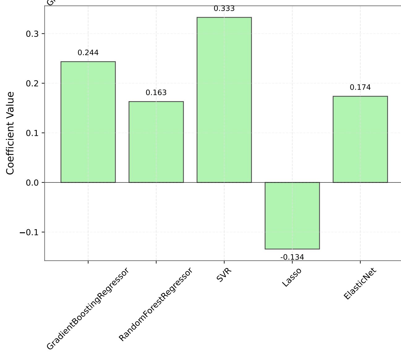
C: Meta-model Coefficients
